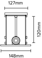
Nicho / Recessed
