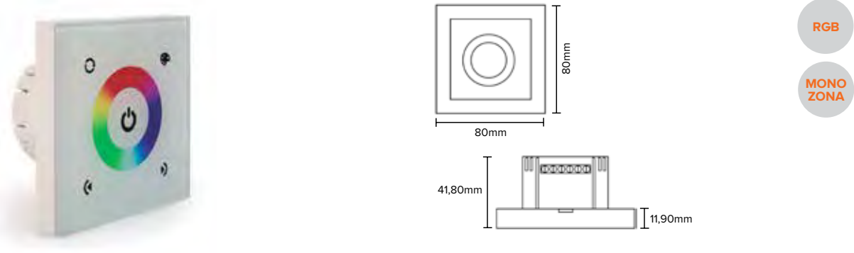
PANEL TÁCTIL MURAL RGB RGB WALL MOUNT TOUCH PANEL
