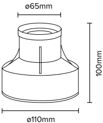
Nicho / Recessed
