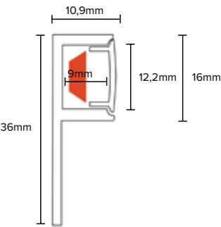
PROFILE TO EMBED IN MINI CONSTRUCTION
