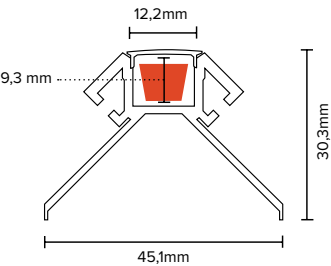
EXTERNAL CORNER ALUMINUM PROFILE
